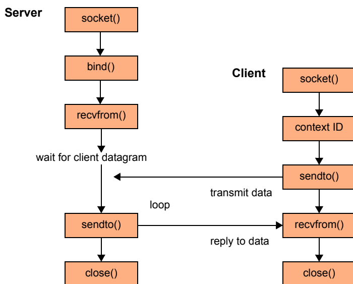
Figure 4-1. Connectionless Datagram Sockets
